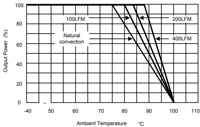
Derating Curve ( 3.3V, 5V & \pm 5V )
