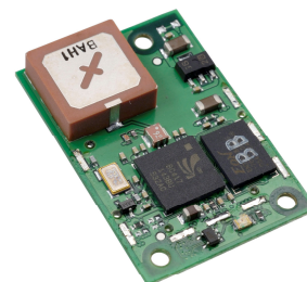
Module shown without RF shield
