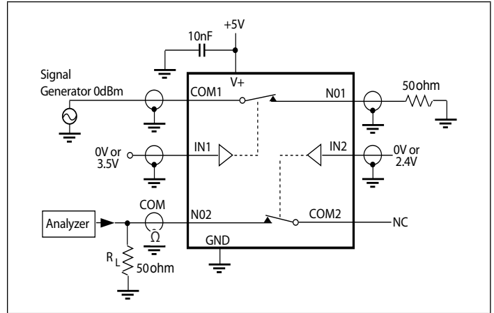
Figure 6. Crosstalk
