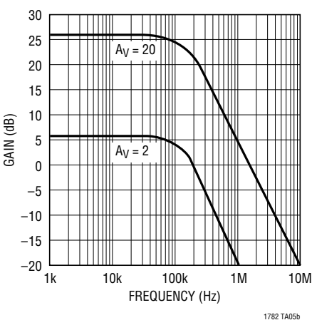
Programmable Gain Amplifier Frequency Response
