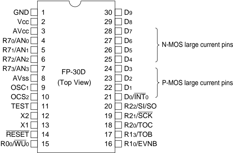
HD404374 Series
