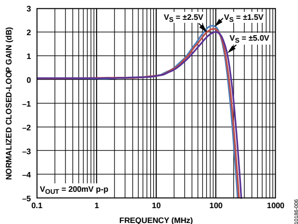
Figure 5. Small Signal Frequency Response vs. Supply Voltage
