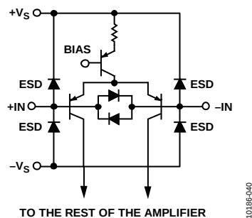
Figure 37. Input Stage and Protection Diodes
