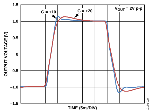
Figure 22. Large Signal Transient Response for Various Gains
