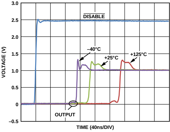
Figure 36. Output Turn-On Time vs. Temperature
