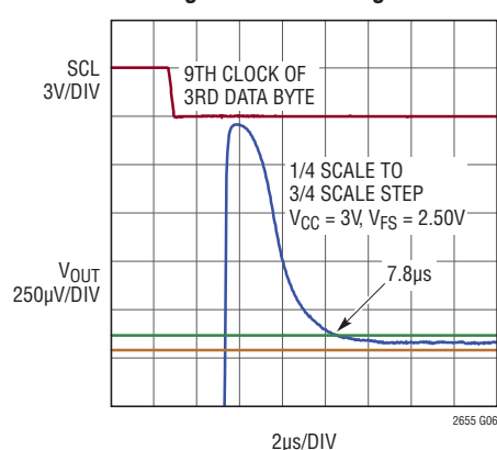
Settling to \pm 1\text{LSB} Rising
