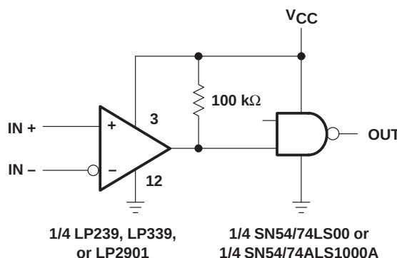
Figure 2. CMOS Driver
