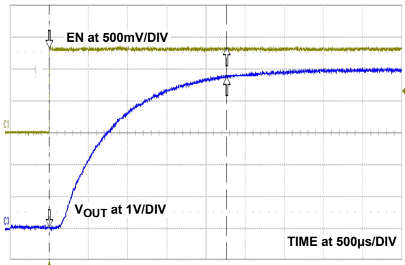
FIGURE 9. START-UP WAVEFORM
