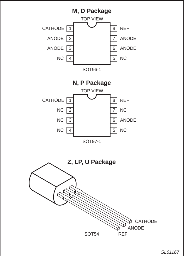
Figure 1. Pin Configuration
