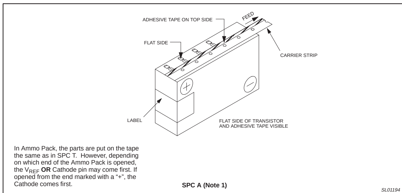
Figure 25. TO-92 Ammo Pack Styles
