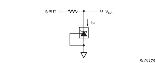
Figure 5. Test Circuit for I_{OFF}
