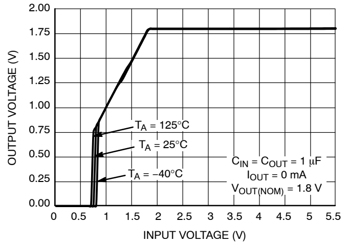
Figure 16. Output Voltage vs. Input Voltage V_{OUT} = 1.8\ \text{V}
