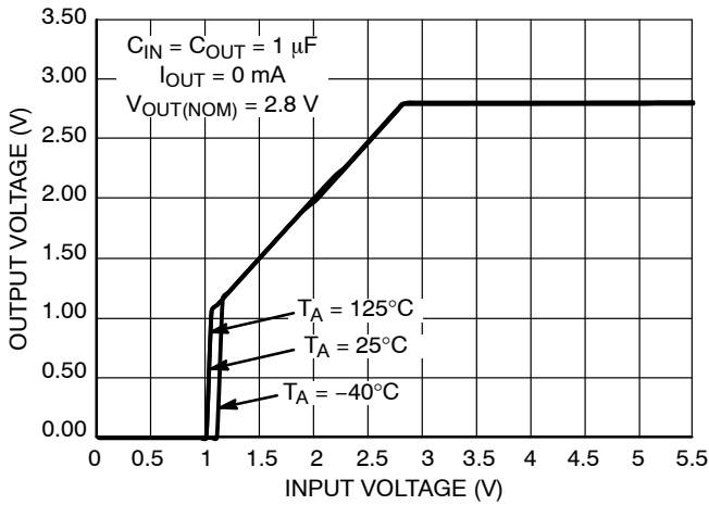
Figure 17. Output Voltage vs. Input Voltage V_{OUT} = 2.8\ \text{V}
