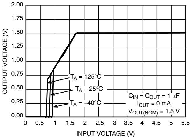
Figure 15. Output Voltage vs. Input Voltage V_{OUT} = 1.5\ \text{V}
