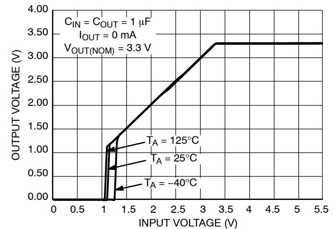
Figure 20. Output Voltage vs. Input Voltage V_{OUT} = 3.3\ \text{V}
