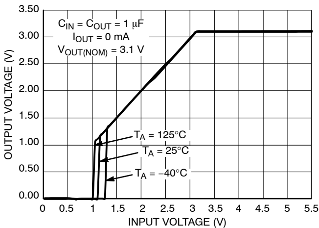
Figure 19. Output Voltage vs. Input Voltage V_{OUT} = 3.1\ \text{V}
