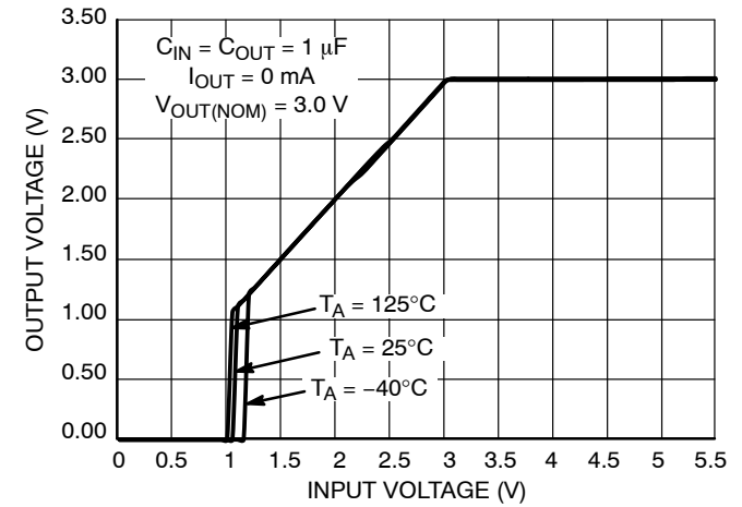
Figure 18. Output Voltage vs. Input Voltage V_{OUT} = 3.0\ \text{V}
