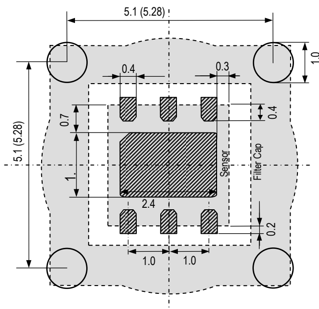
Figure 3: PCB layout of SHT2x and Filter Cap SF2. Dimensions are given in mm (1mm = 0.039 inch). The distance of the openings is 5.1mm \pm 0.05mm if the sensor should clip on the PCB and 5.28mm if the pins are used for adjustment only. By varying the openings distance about \pm 0.05mm the clipping force may be adjusted.
