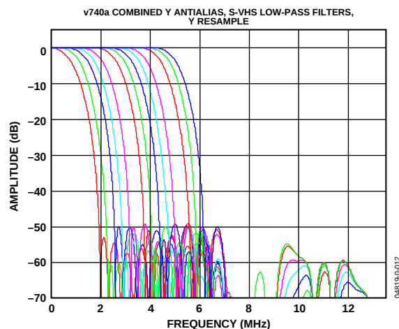
Figure 11. SDP Y S-VHS Combined Responses
