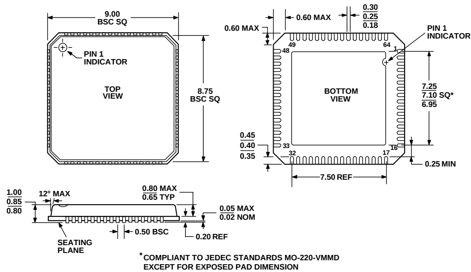
Figure 42. 64-Lead Lead Frame Chip Scale Package [LFCSP] 9 mm × 9 mm Body (CP-64-3)
