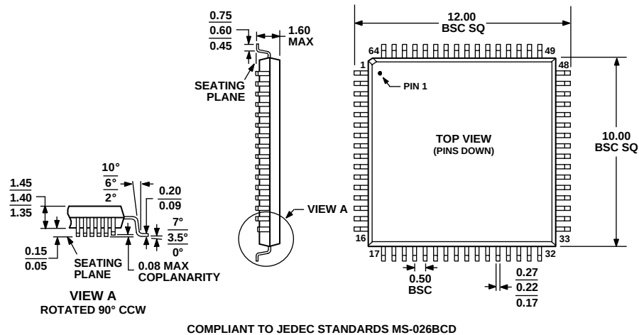
Figure 43. 64-Lead Low Profile Quad Flat Package [LQFP] (ST-64-2)
