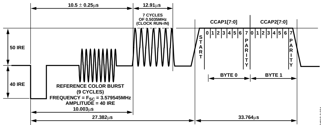
Figure 33. SDP Closed Caption Data Extraction
