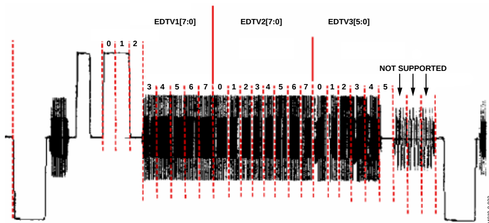
Figure 31. SDP EDTV Data Extraction
