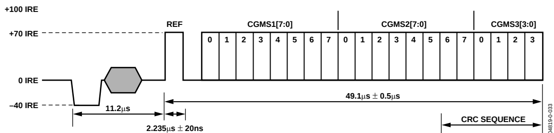
Figure 32. SDP CGMS Data Extraction
