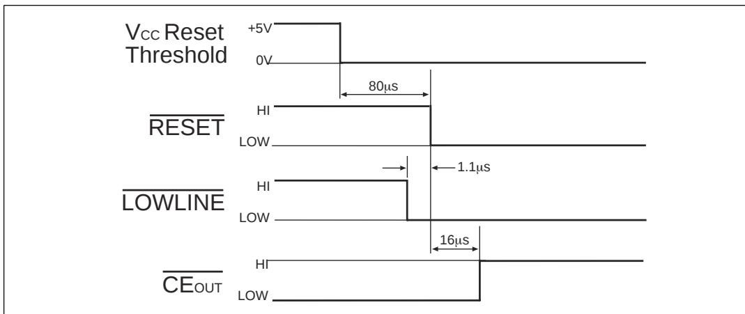
Figure 15. V_{CC} to LOWLINE and \overline{CE}_{OUT} Delay
