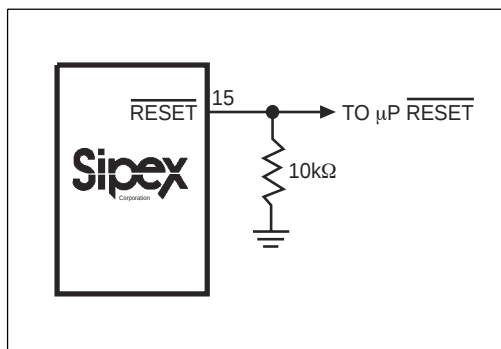
Figure 18. External Pull-down Resistor Ensures \overline{\text{RESET}} is Valid with V_{CC} Down to Ground.
