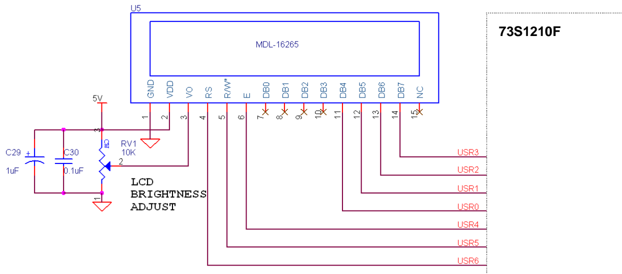
Figure 16: LCD Connections
