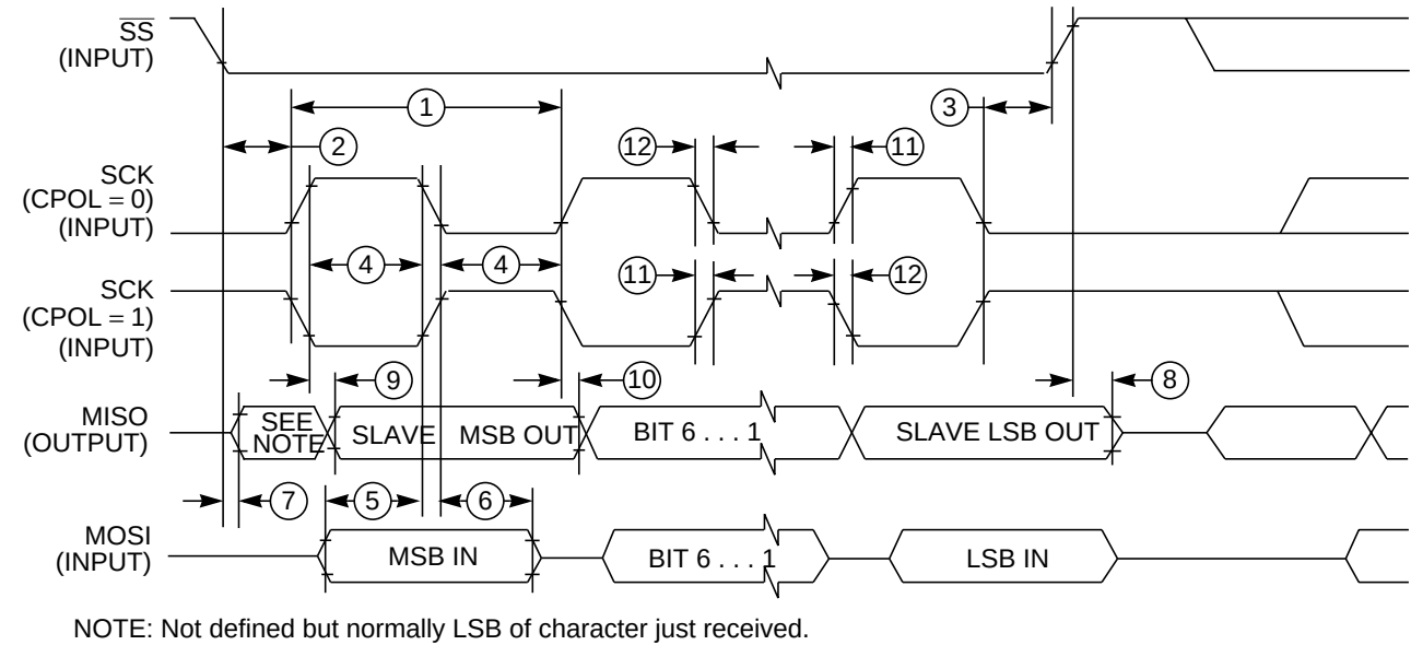
Figure A-8 SPI Slave Timing (CPHA = 1)
