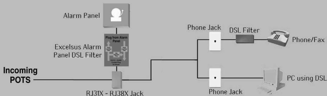
Block Schematic
