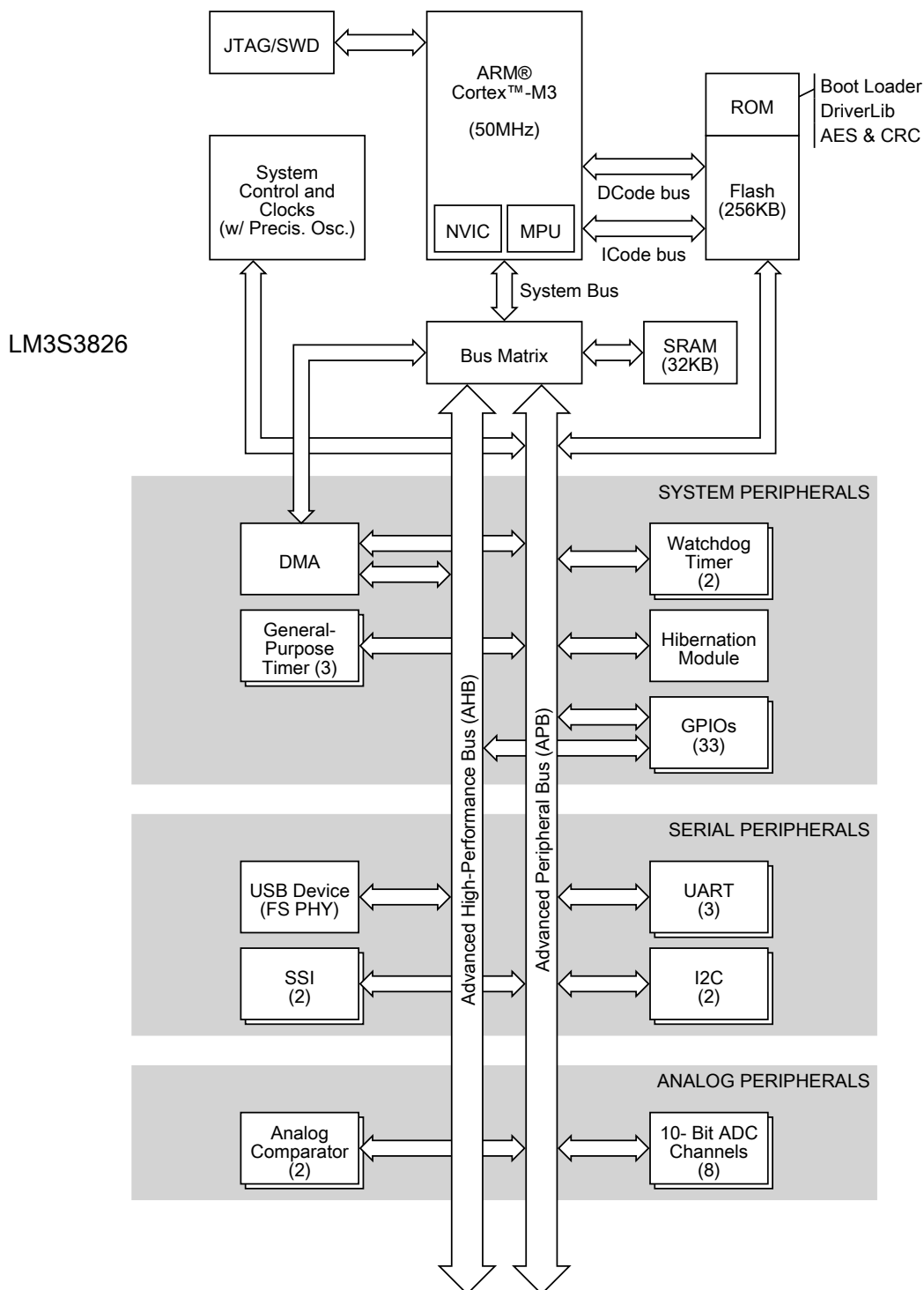
Figure 1-1. Stellaris LM3S3826 Microcontroller High-Level Block Diagram
