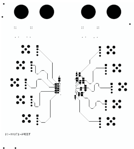
Figure 11. Signal Traces On Bottom Layer
