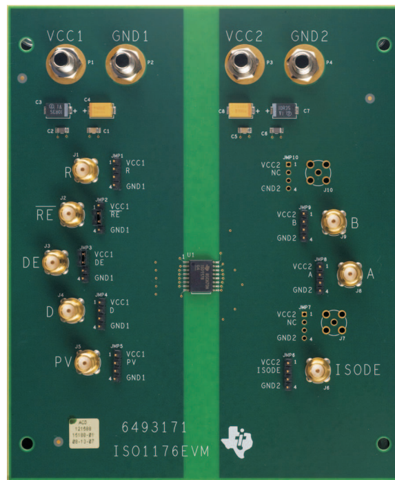
Figure 2. The ISO1176EVM
