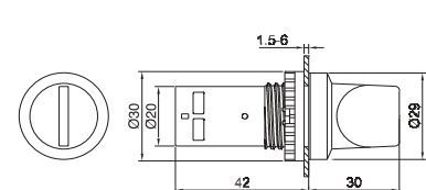
Selector switch
