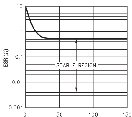
Figure 31. 2.2- \mu\text{F} /3.3- \mu\text{F} Stable ESR Range for Output Voltage \geq 2.5 V
