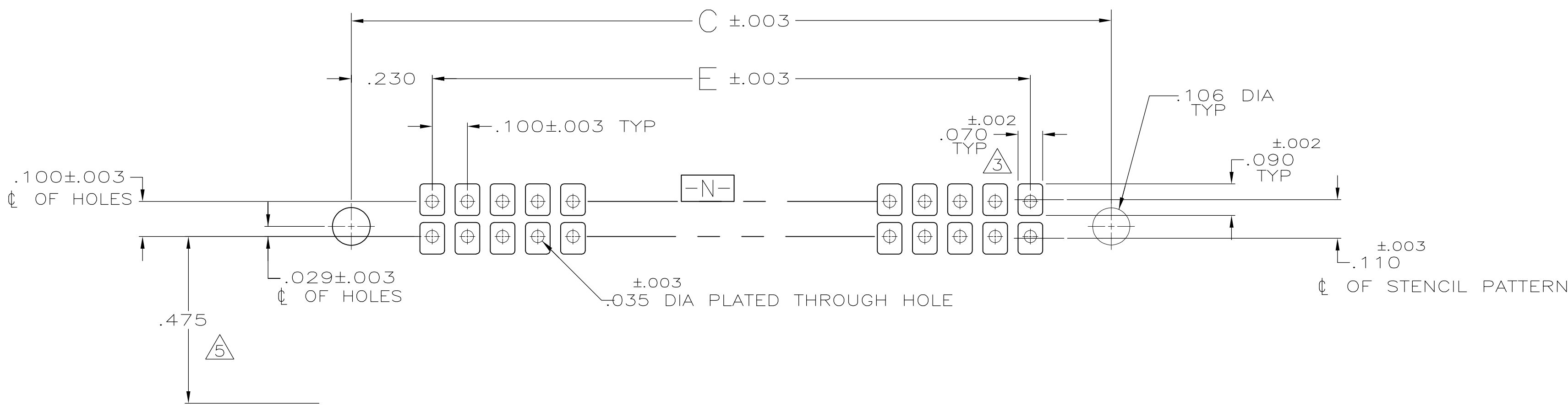
SECTION Z-Z
