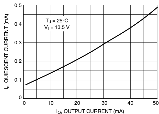
Figure 28. Quiescent Current vs. Output Current (Low Load)
