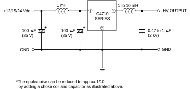
Figure 3: Example of Ripple / Noise Reduction Circuit
