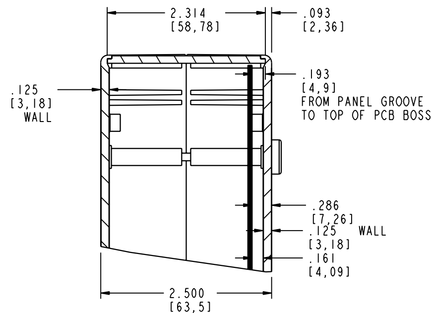
SECTION C-C
