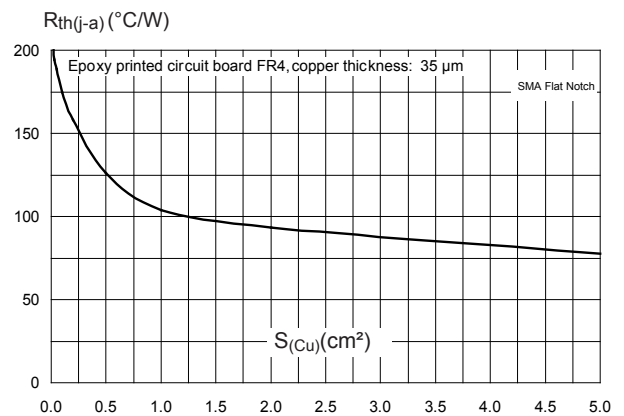
Figure 10. Thermal resistance junction to ambient versus copper surface under each lead (SMA Flat Notch)
