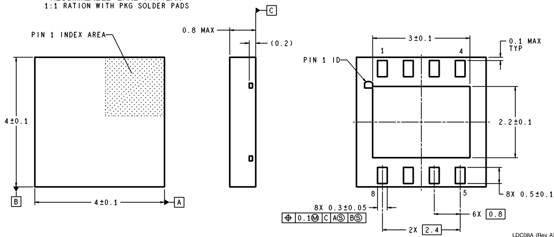
8-Lead LLP Surface Mount Package NS Package Number LDC08A
