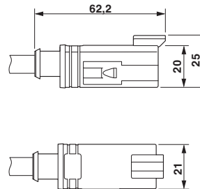
DEUTSCH DT04-3P, top view and side view
