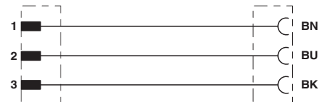
Contact assignment of the DEUTSCH connectors
