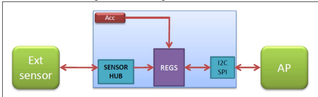
Figure 13. Block diagram of sensor hub
