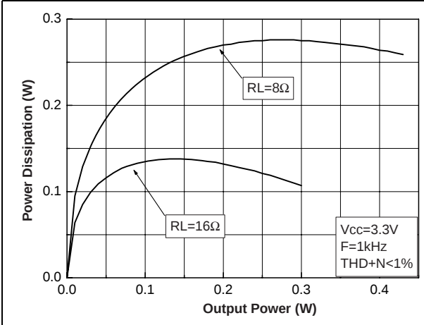
Figure 9. Power dissipation vs. output power
