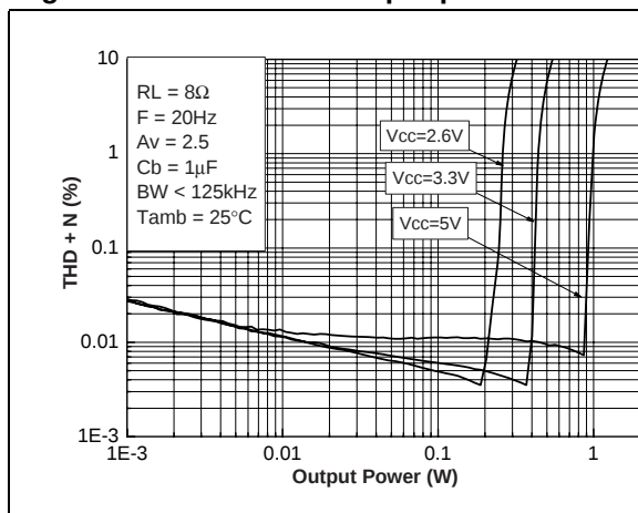
Figure 43. THD+N vs. output power
