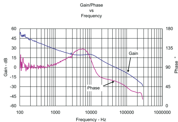
Figure 7-6. TPS40195EVM Bode Plot V_{IN} = 12\text{ V} , I_{OUT} = 20\text{ A} , Crossover Frequency = 48 kHz, Phase Margin = 57.5°
