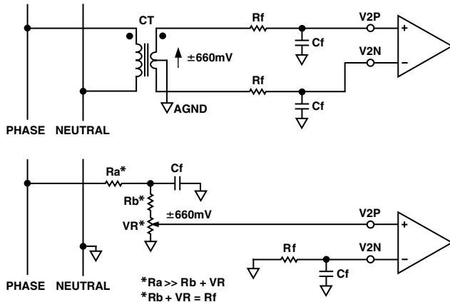
Figure 25. Typical Connections for Channel V2
