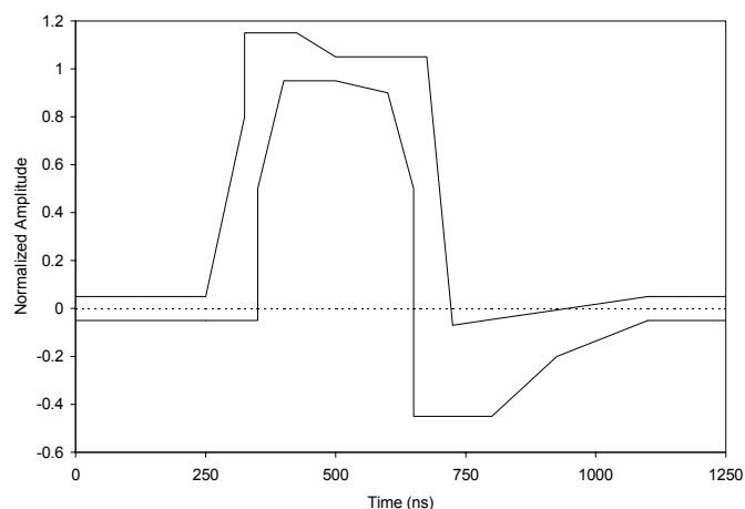
Figure-9 DSX-1 Waveform Template
