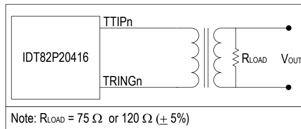
Figure-12 E1 Waveform Template Measurement Circuit
