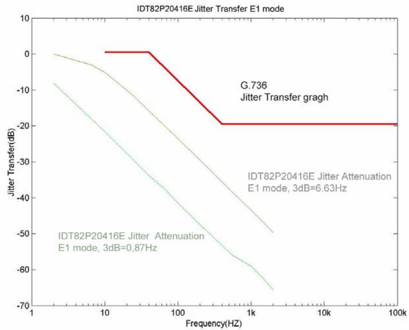
Figure-43 E1 Jitter Transfer Performance
