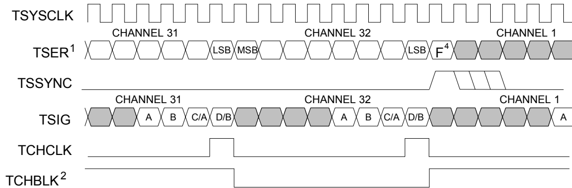
Figure 13-12. T1 Transmit-Side 2.048MHz Boundary Timing (Elastic Store Enabled)
