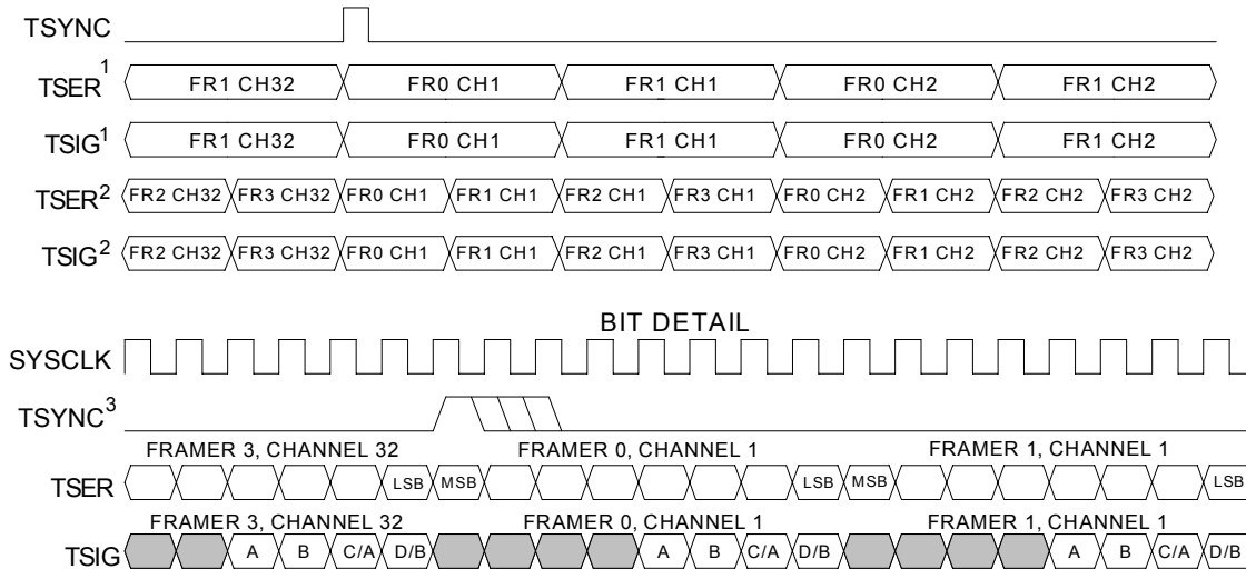
Figure 13-13. T1 Transmit-Side Interleave Bus Operation, BYTE Mode
