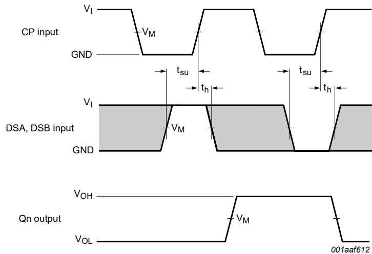
Measurement points are given in Table 8. The shaded areas indicate when the input is permitted to change for predictable output performance. V_{OL} and V_{OH} are typical voltage output levels that occur with the output load.
