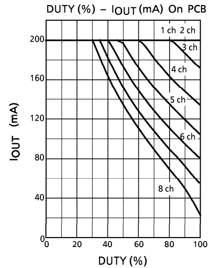
Fig.5 DUTY - I_{OUT} ( T_{opr} = 25^\circ\text{C} )
