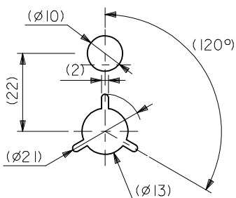
DETAIL "H"
