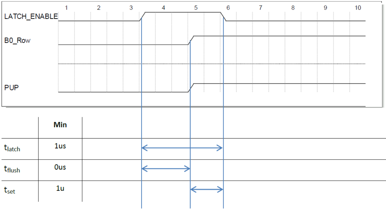
Figure 7: Device control
