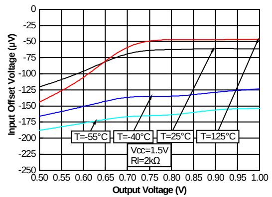
Figure 5: Input offset voltage vs output voltage at V_{CC} = 1.5\text{ V}
