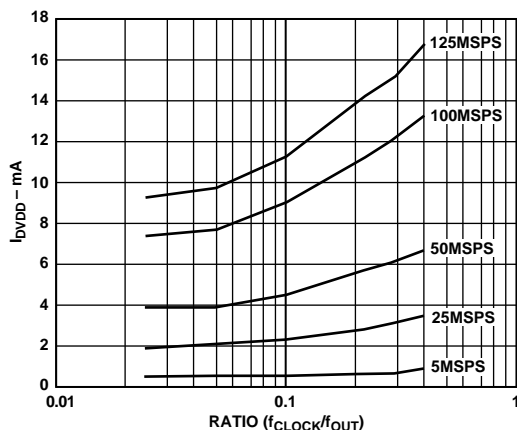
Figure 26. I_{DVDD} vs. Ratio @ DVDD = 5\text{ V}
