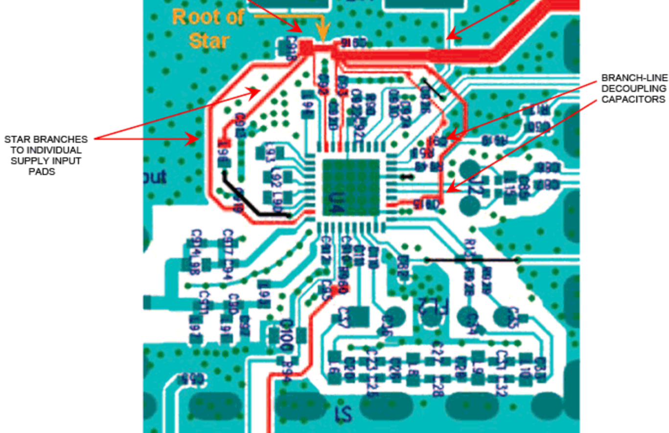
Figure 9. If a component has several supply connections, the power-supply routes can be arranged in a star configuration.
