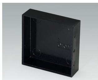
A8050160 POTTING BOXES, Vers. I PF (UL 94 V-0) black RAL 9005 1.97"x1.97"x0.59"
