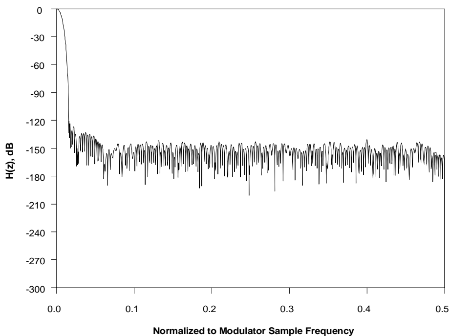
Modulator Sample Frequency = MCLK/16; Output Word Rate = MCLK/2048 Hz Digital Filter Total Response
