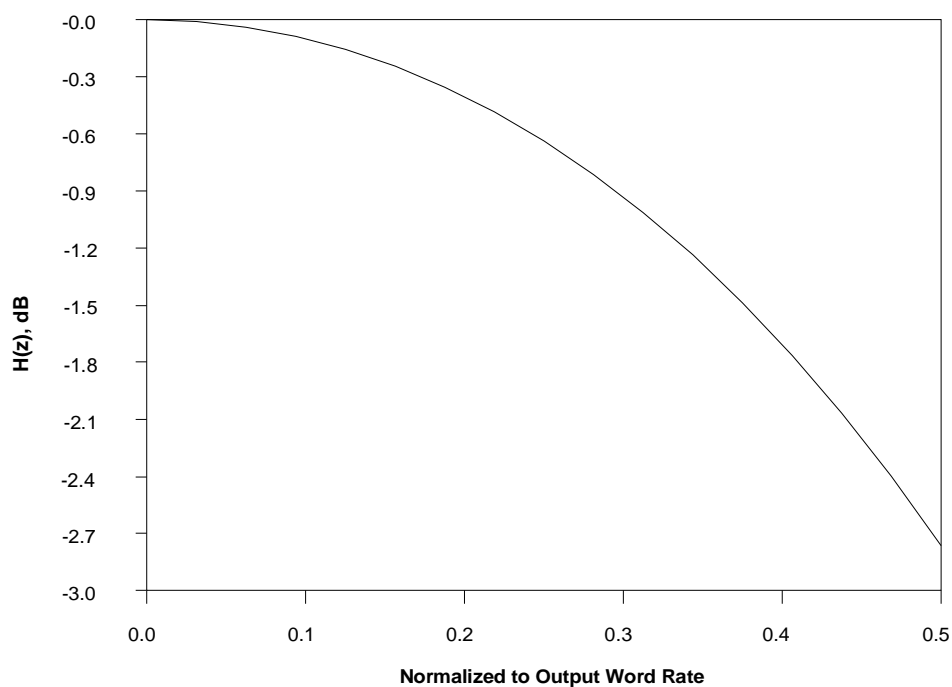
CS5543 Digital Filter Passband Response
