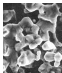
Figure 2. Sintered Anode
