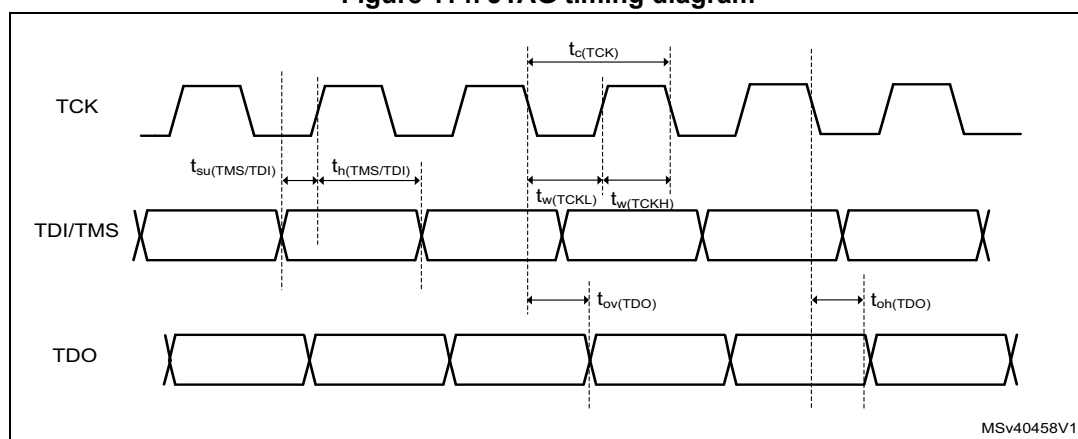
Figure 114. JTAG timing diagram
