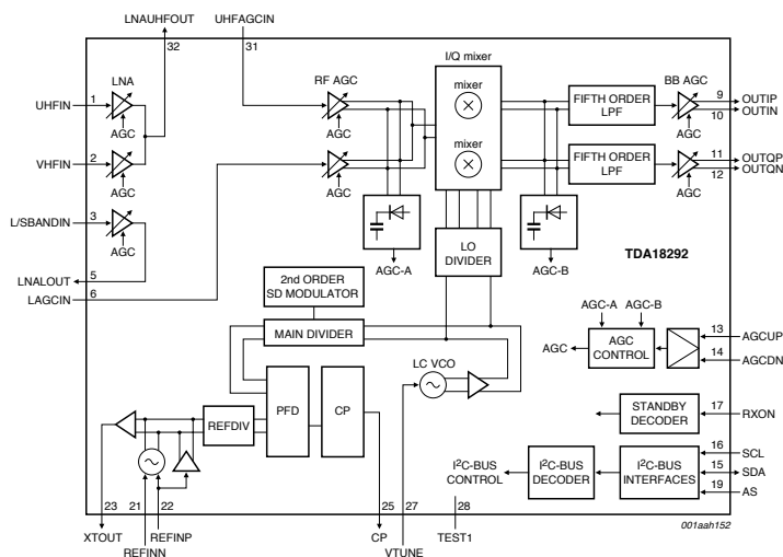
TDA18292 block diagram
