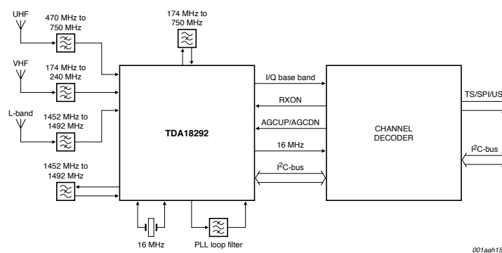
System level block diagram
