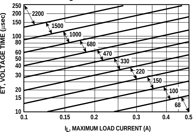
Figure 40. TC2574-ADJ
