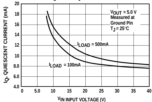
Figure 27. Quiescent Current
