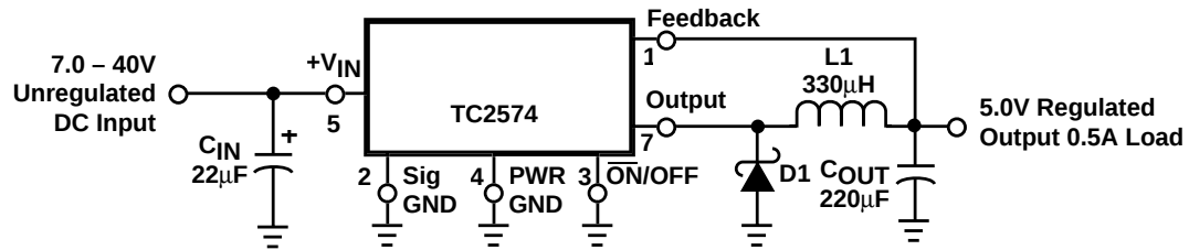
Figure 1. Block Diagram and Typical Application: Fixed Output Versions
