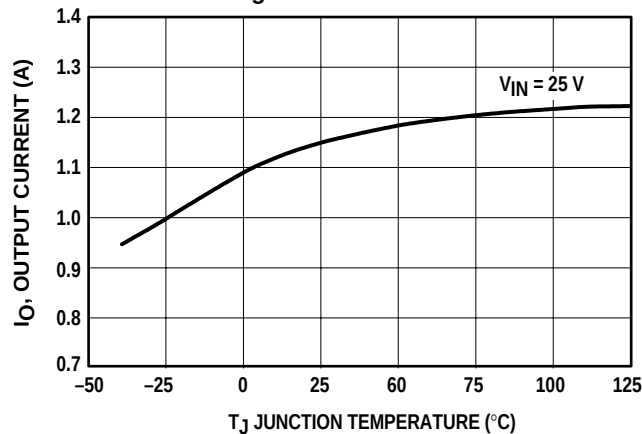
Figure 26. Current Limit
