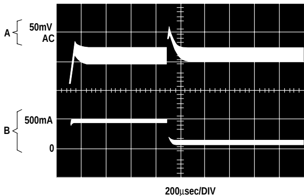
Figure 35. 500mA Load Transient Response for Continuous Mode Operation, L = 330\mu\text{H} , C_{\text{OUT}} = 300\mu\text{F}
