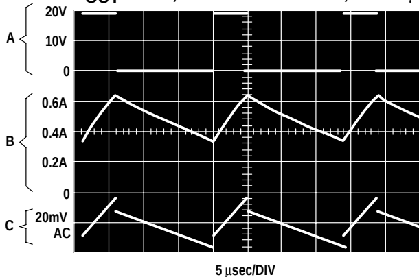
Figure 33. Continuous Mode Switching Waveforms V OUT = 5.0V, 500mA Load Current, L = 330μH
