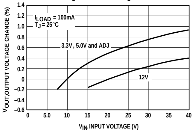
Figure 24. Line Regulation
