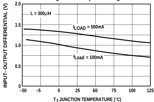
Figure 25. Dropout Voltage
