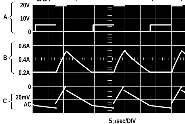
Figure 34. Discontinuous Mode Switching Waveforms V OUT = 5.0V, 100mA Load Current, L = 100μH
