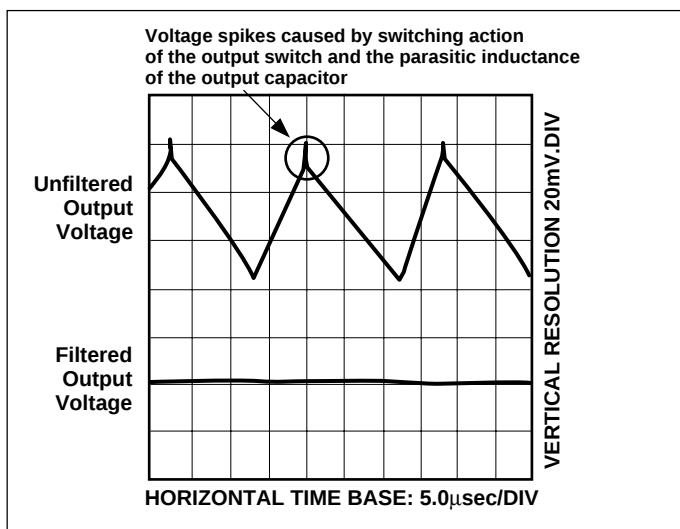
Figure 7. Output Ripple Voltage Waveforms
