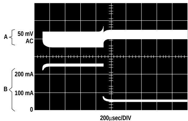
Figure 36. 250mA Load Transient Response for Discontinuous Mode Operation, L = 68\mu\text{H} , C_{\text{OUT}} = 470\mu\text{F}
