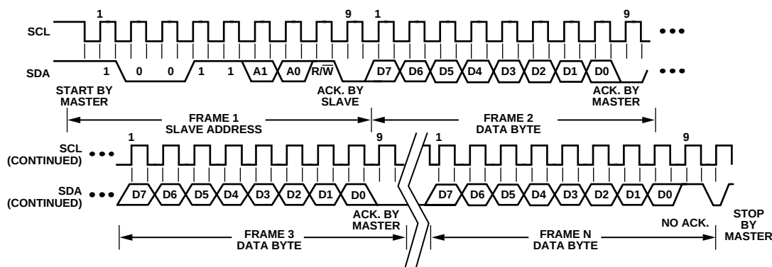
Figure 36. General SMBus Read Timing Diagram
