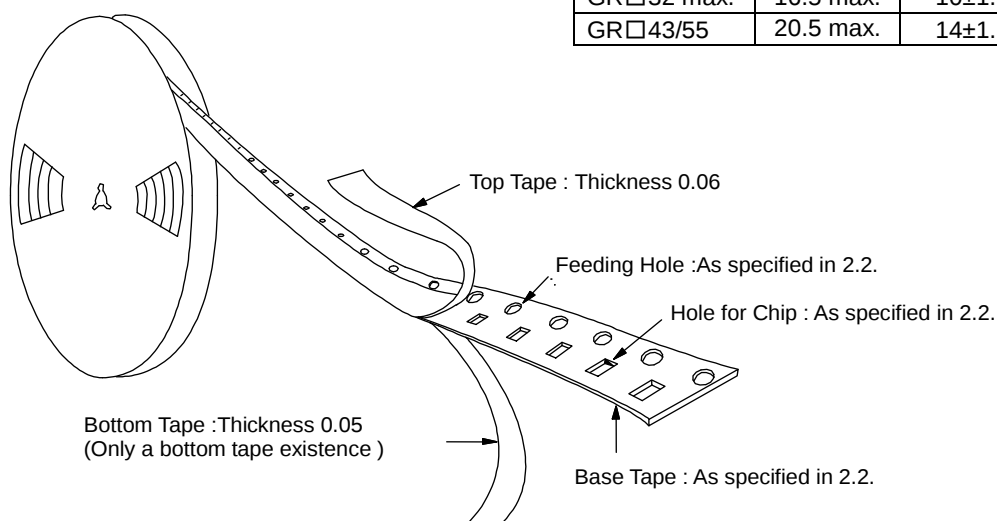
Fig.3 Taping Diagram
