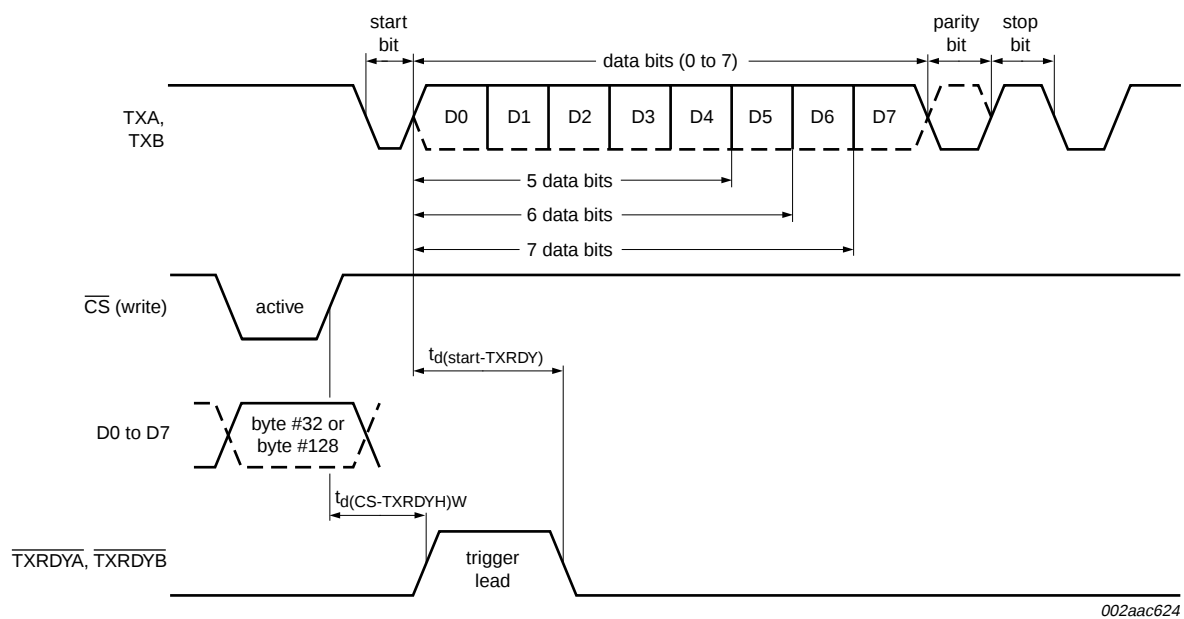
Fig 29. Transmit ready timing in FIFO mode (DMA mode '1') in 68 mode
