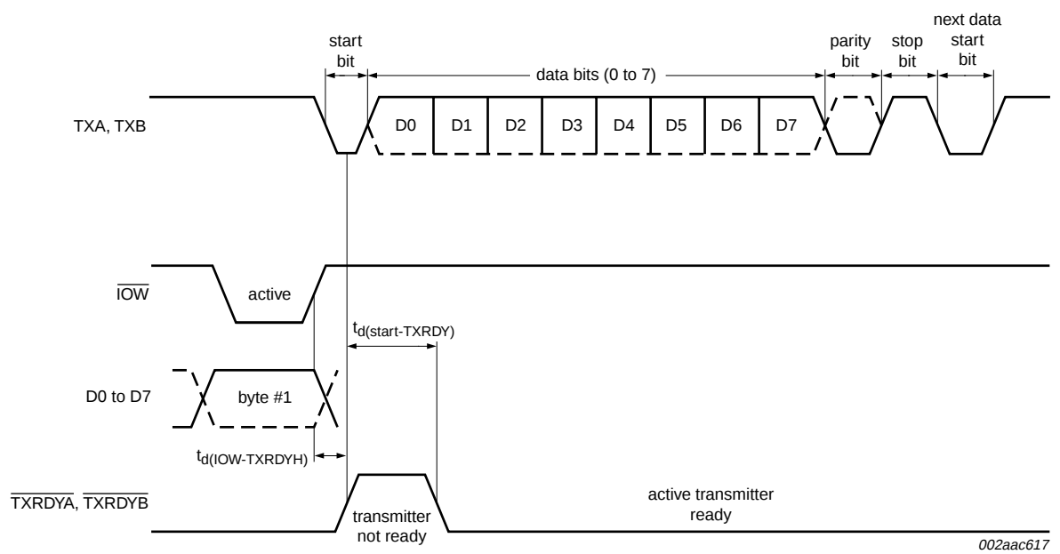
Fig 26. Transmit ready timing in non-FIFO mode (16 mode)
