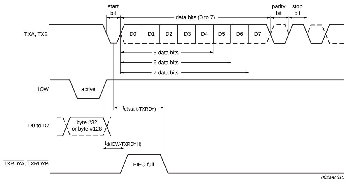
Fig 28. Transmit ready timing in FIFO mode (DMA mode '1') in 16 mode
