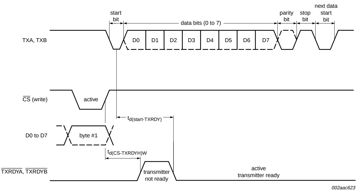
Fig 27. Transmit ready timing in non-FIFO mode (68 mode)
